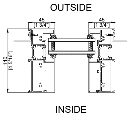
110 FIXED Horizontal Section
