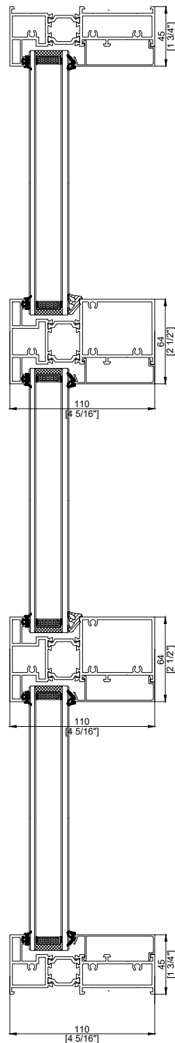
110 FIXED DIRECT HORIZONTAL MULL Vertical Section
