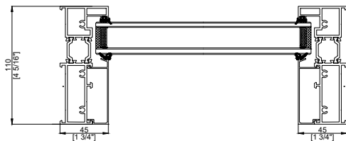
110 FIXED Horizontal Section
