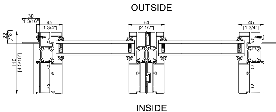
110 FIXED DIRECT VERTICAL MULL Horizontal Section
