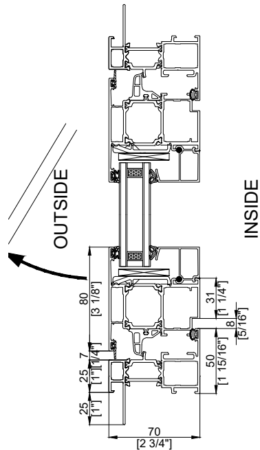
70 AWNING Vertical Section
