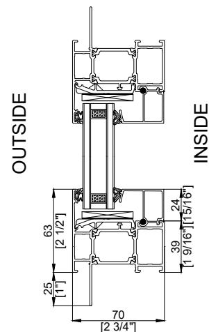
70 FIXED Vertical Section
