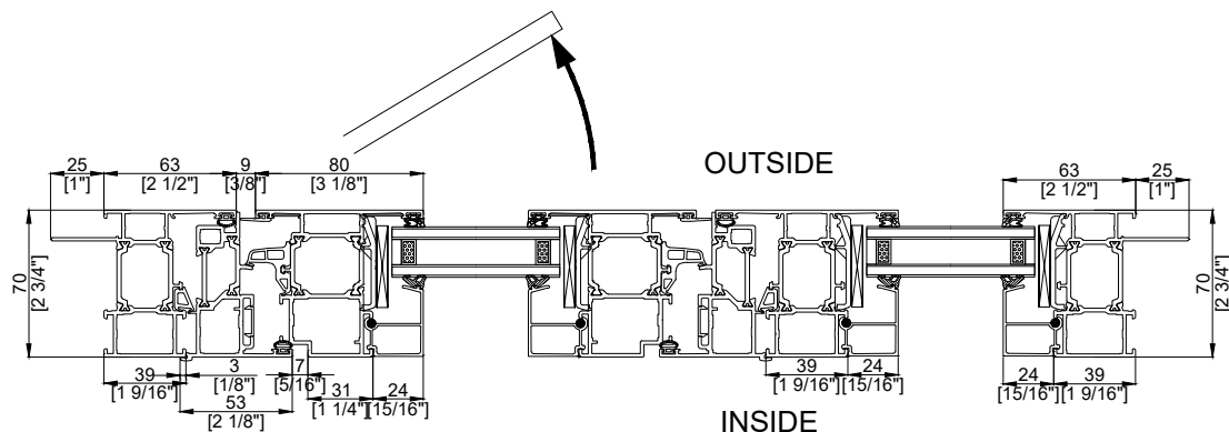
70 PUSH OUT CASEMENT Vertical Section
