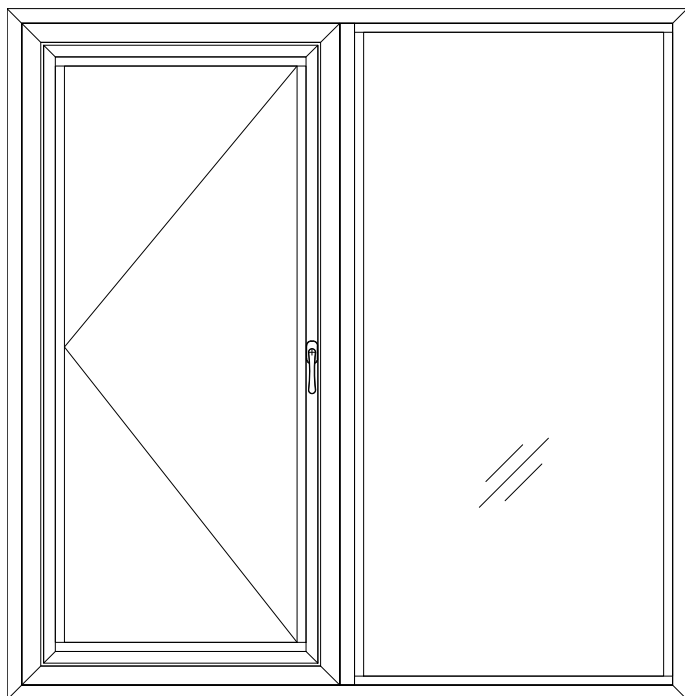
70 PUSH OUT CASEMENT - FIXED DIRECT VERTICAL MULL Elevation View (Interior)
