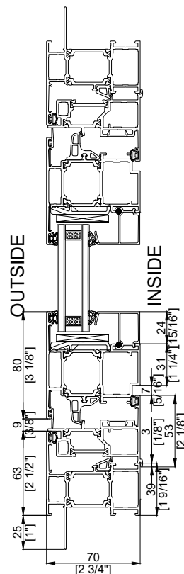
70 PUSH OUT CASEMENT Vertical Section
