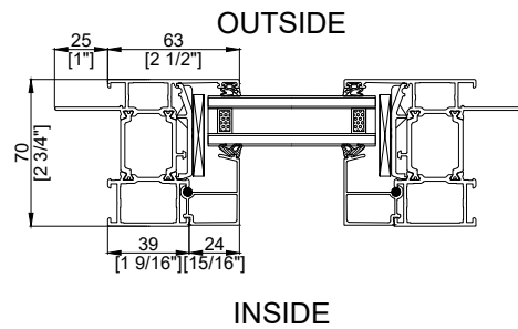
70 FIXED Horizontal Section
