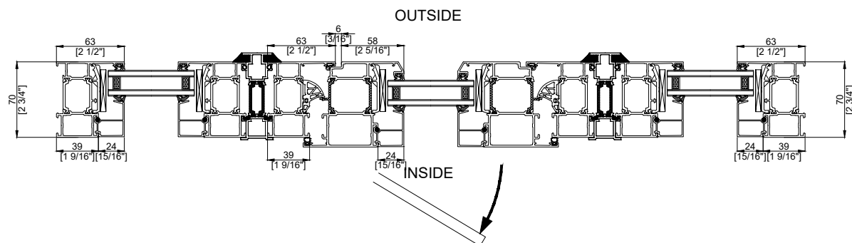
70 SERIES ENTRY INSWING & FIXED MULL Horizontal Section
