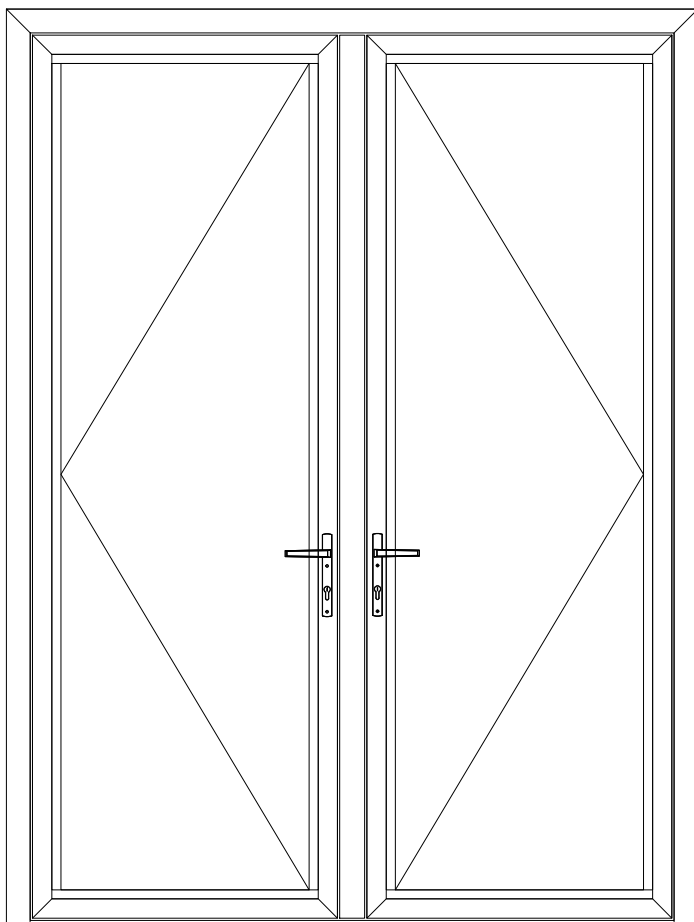
70 SERIES ENTRY OUTSWING FRENCH DOOR Elevation View
