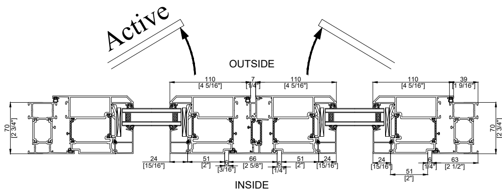
70 SERIES ENTRY OUTSWING FRENCH DOOR Horizontal Section
