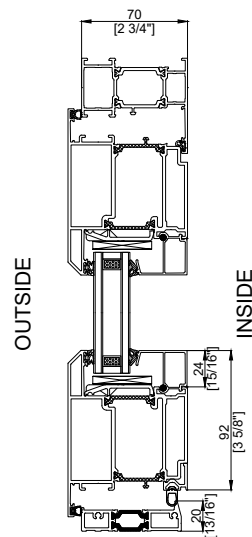
70 SERIES ENTRY OUTSWING Vertical Section
