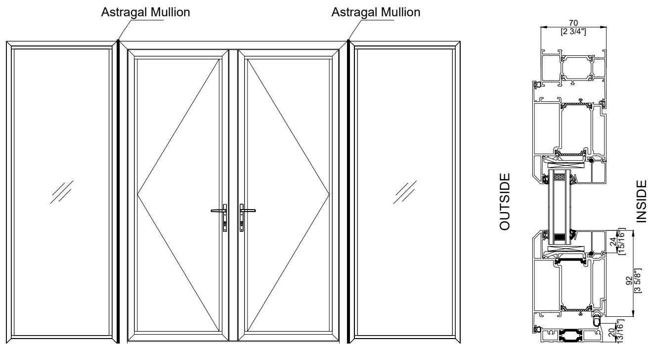
70 SERIES ENTRY OUTSWING Vertical Section
