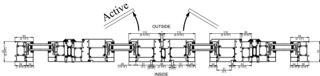
70 SERIES ENTRY OUTSWING & FIXED MULL Horizontal Section
