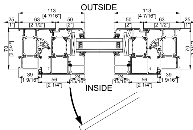
70 TILT / TURN Horizontal Section
