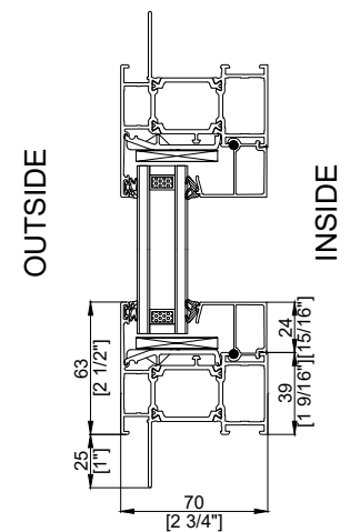
70 FIXED Vertical Section
