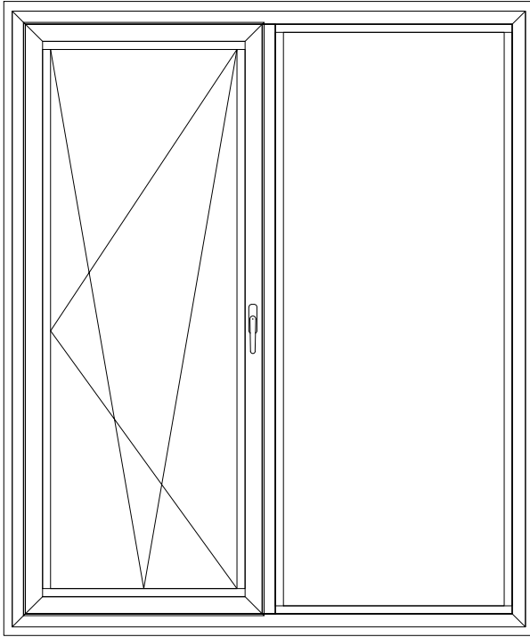
70 TILT / TURN - FIXED DIRECT VERTICAL MULL Elevation View (Interior)
