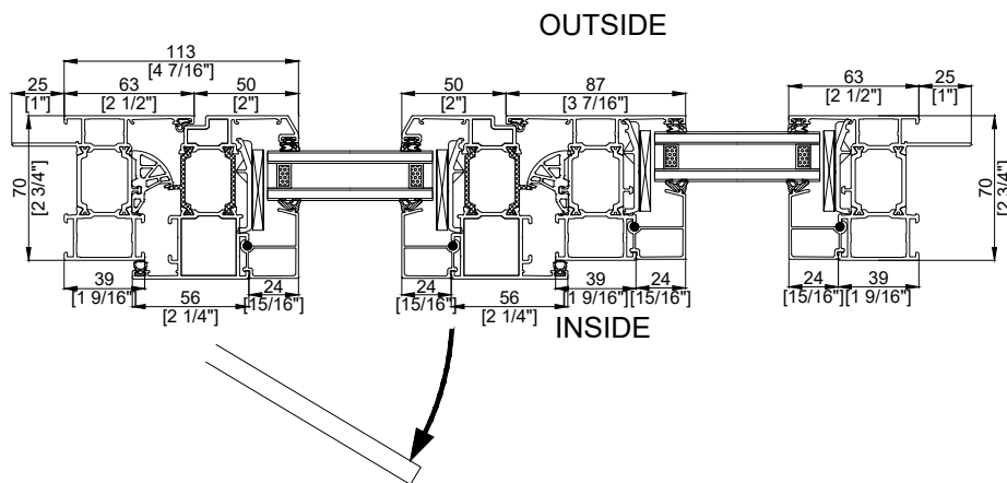
70 TILT / TURN - FIXED DIRECT VERTICAL MULL Horizontal Section
