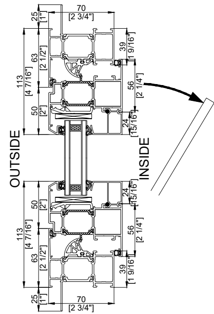
70 TILT / TURN Vertical Section
