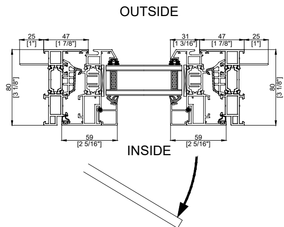
80 TILT / TURN Horizontal Section
