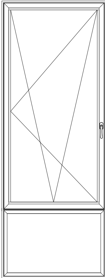
80 TILT / TURN - FIXED DIRECT HORIZONTAL MULL Elevation View (Interior)
