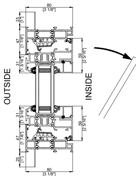
80 TILT / TURN Vertical Section
