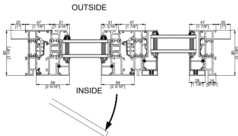
80 TILT / TURN - FIXED DIRECT VERTICAL MULL Horizontal Section
