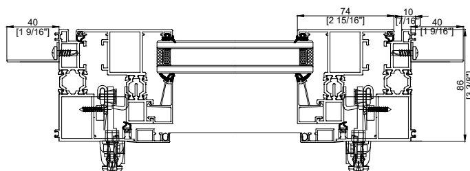
86 AWNING Horizontal Section
