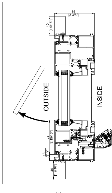
86 AWNING Vertical Section
