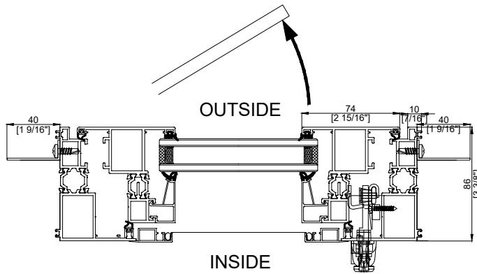
86 CRANK CASEMENT Horizontal Section
