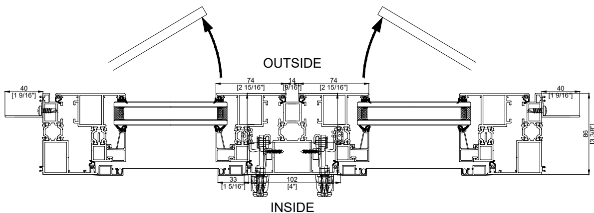
86 CRANK CASEMENT DIRECT VERTICAL MULL Horizontal Section
