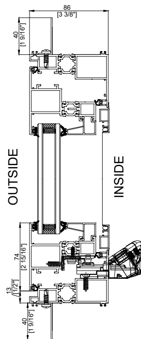
86 CRANK CASEMENT Vertical Section
