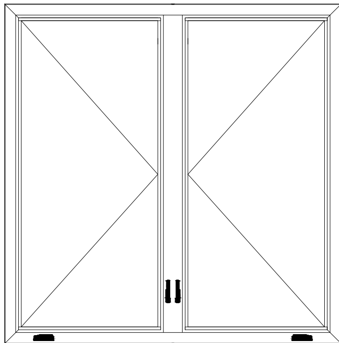
86 CRANK CASEMENT DIRECT VERTICAL MULL Elevation View (Interior)
