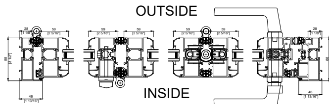
ONE WAY BIFOLD 3 PANEL Horizontal Section
