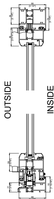
BIFOLDING DOOR Vertical Section
