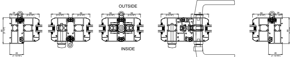
TWO-WAY BIFOLD 4 PANEL Horizontal Section
