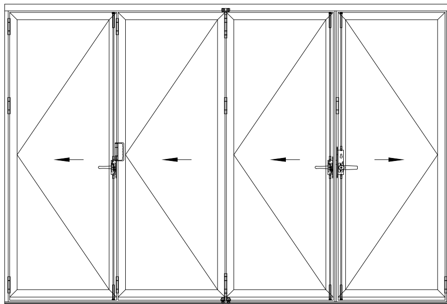
TWO-WAY BIFOLD 4 PANEL Elevation View
