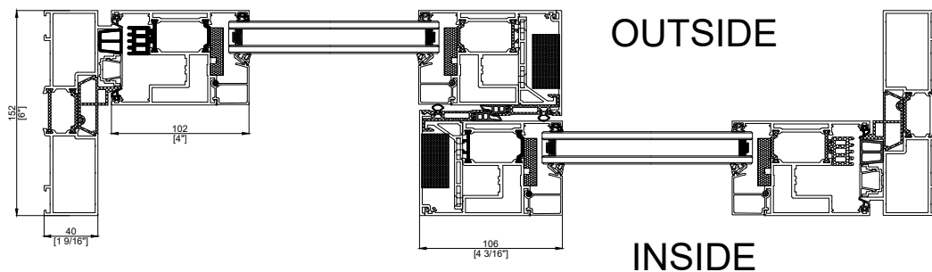
LIFT AND SLIDE STANDARD Horizontal Section
