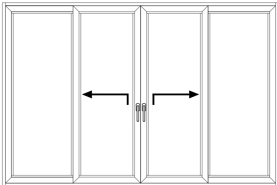
LIFT AND SLIDE BIPARTING Elevation View
