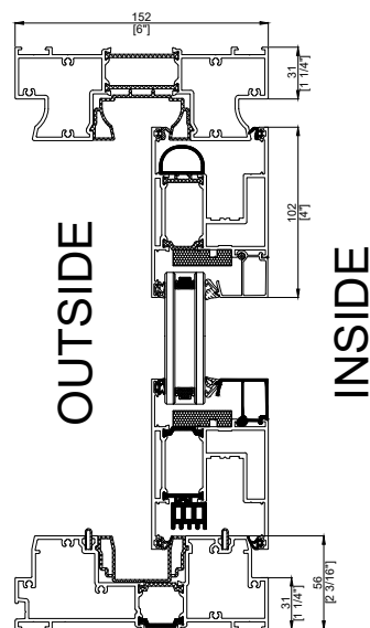
LIFT AND SLIDE / STANDARD SILL Vertical Section
