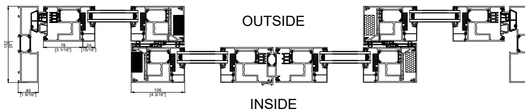
LIFT AND SLIDE BIPARTING Horizontal Section
