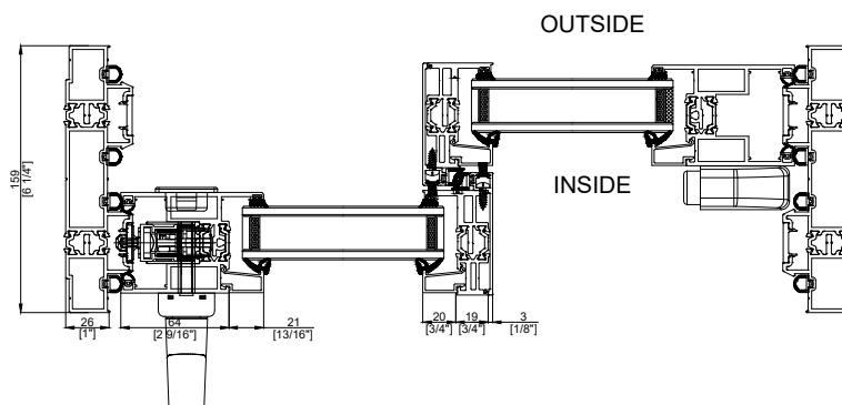
LIFT AND SLIDE SLIM LINE Horizontal Section
