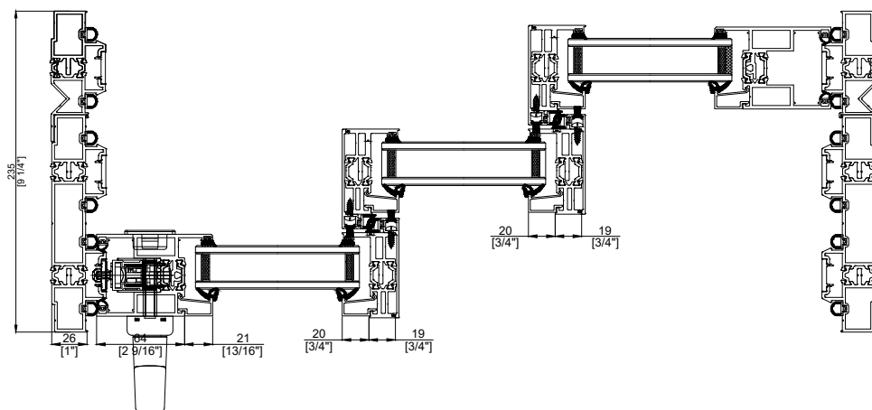
LIFT AND SLIDE SLIM LINE TRIPLE Horizontal Section
