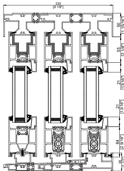
LIFT AND SLIDE SLIM LINE TRIPLE Vertical Section
